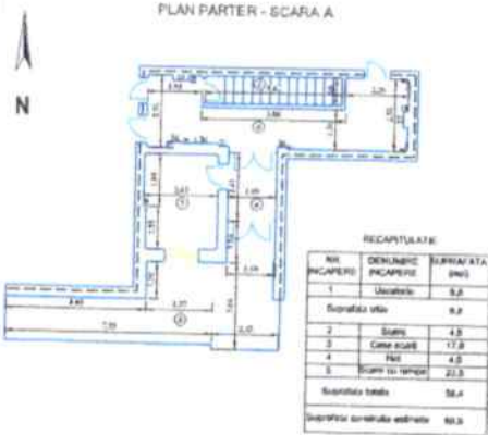
PLAN PARTER - SCARA A
